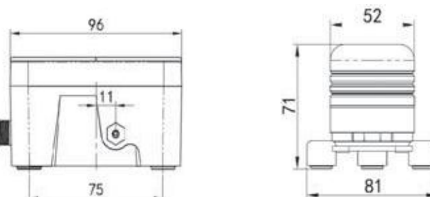
Alarm Box
